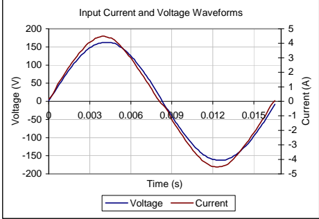
Input AC Current Waveform (I THD = 7.62%, 50% Load)
