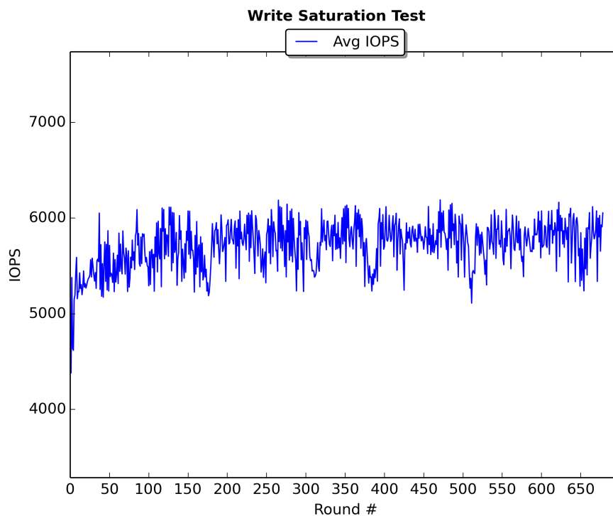
The Write Saturation IOPS Plot shows the average IOPS of 4k random writes over all rounds.
